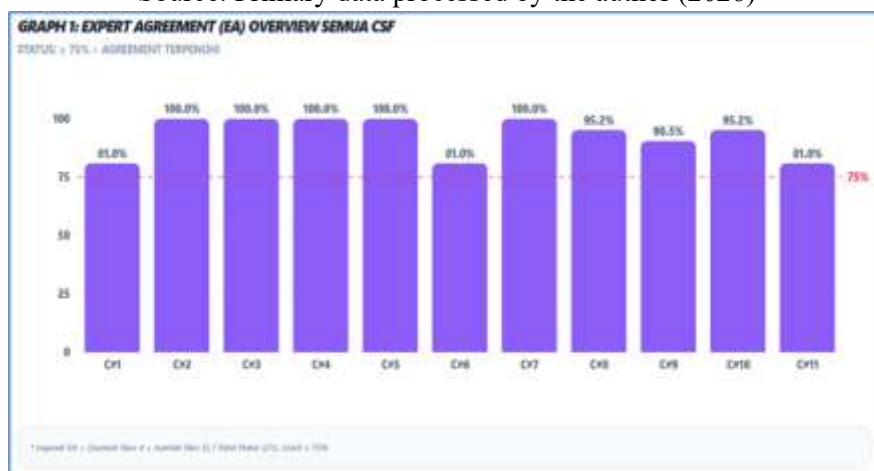
Figure 2. Test Result Graph % Expert Agreement for all CSF#i
