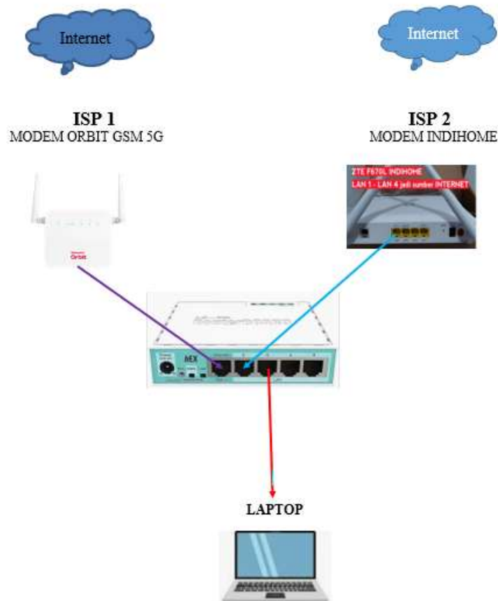
Figure 1. Network Topology
