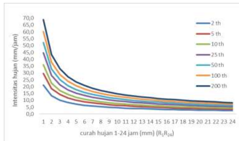
Figure 2. Rainfall Intensity Graph for 2 years – 200 years
