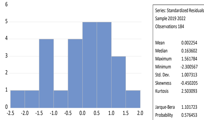
Figure 1. Normality Test
