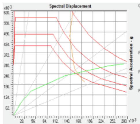
Figure 3. Pushover Analysis
