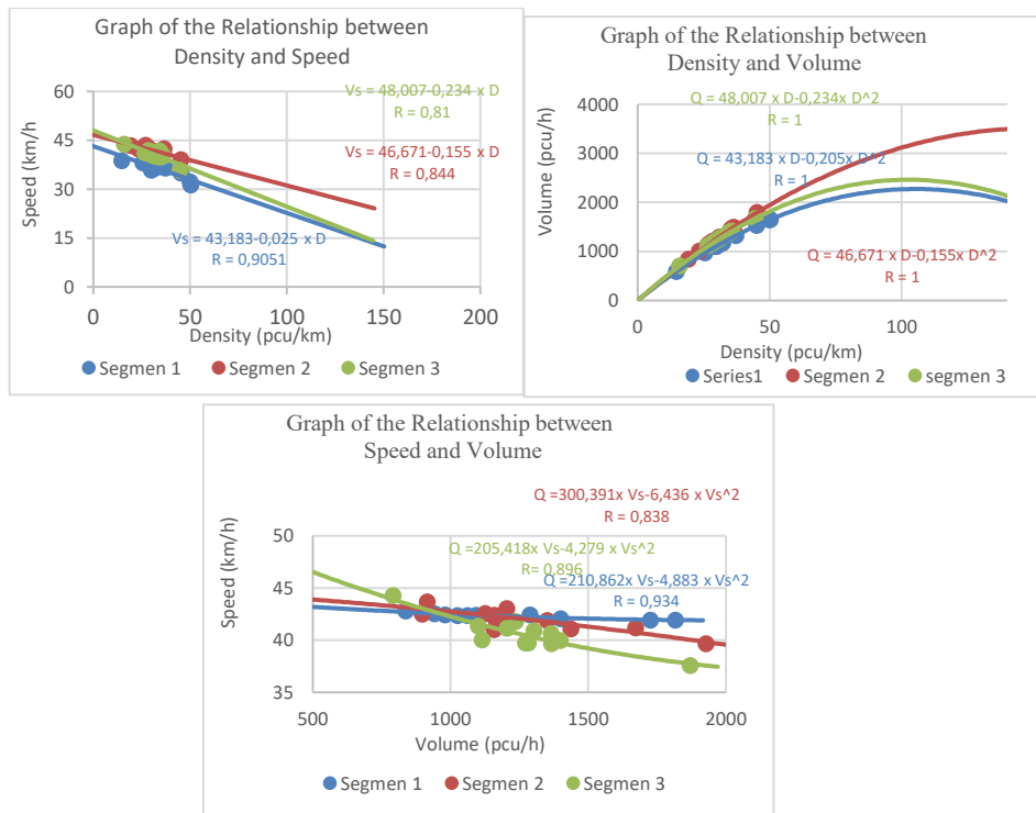
Figure 2. Graph of the Relationship Between V_s - D , Q - D , Q - V_s , With Greensfield's Model, Segments 1, 2, and 3
