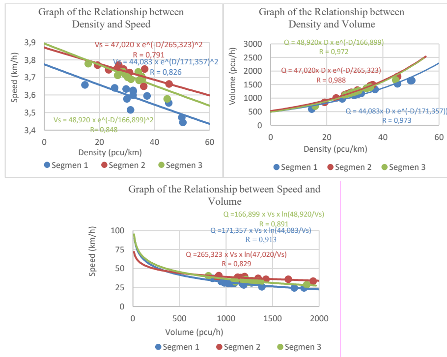
Figure 4. Graph of the Relationship Between Vs – D, Q – D, Q – Vs, With Underwood's Model, Segments 1, 2, and 3
