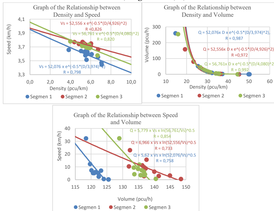
Figure 4. Graph of the Relationship Between Vs – D, Q – D, Q – Vs, With Underwood's Model, Segments 1, 2, and 3
